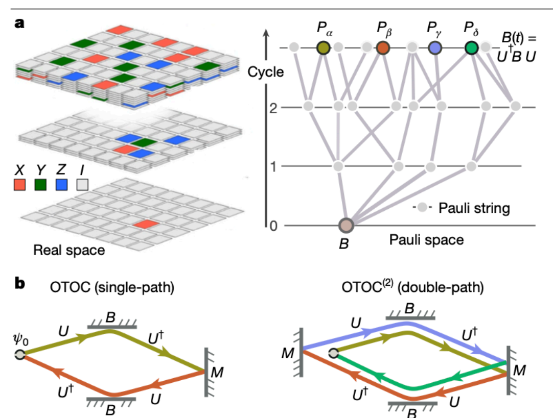
Fig. 1 | OTOCs as interferometers. a , When dynamical protocols involve echoing, the Heisenberg picture of the operator evolution is the natural framework for studying dynamics. b , OTOC and OTOC (2) can be viewed as time interferometers, which highlights their capability of refocusing on desired details and echoing out unwanted dynamics. See text for the definition of parameters.
