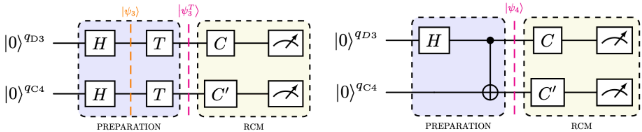
(c) Separable two-qubit states. (d) Bell state.
