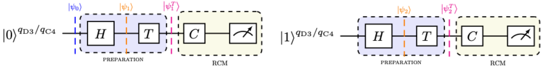
(a) Single-qubit state initially in the |0\rangle state. (b) Single-qubit state initially in the |1\rangle state.
